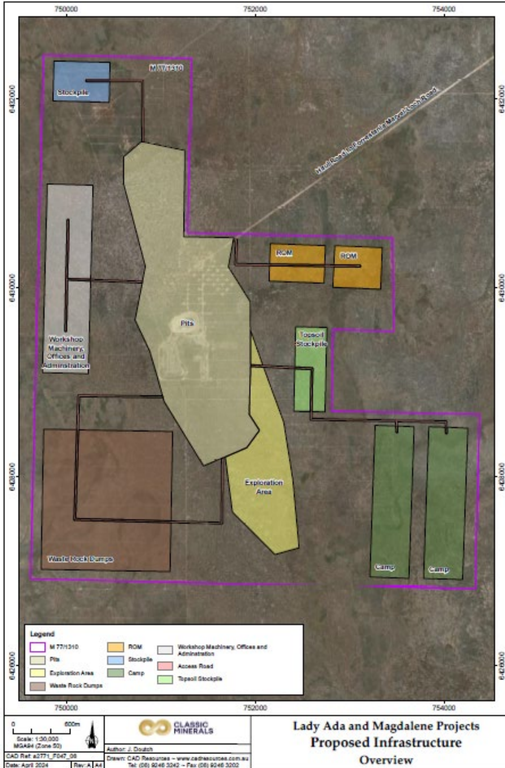
Figure 3: Proposed Mine Site Layout
